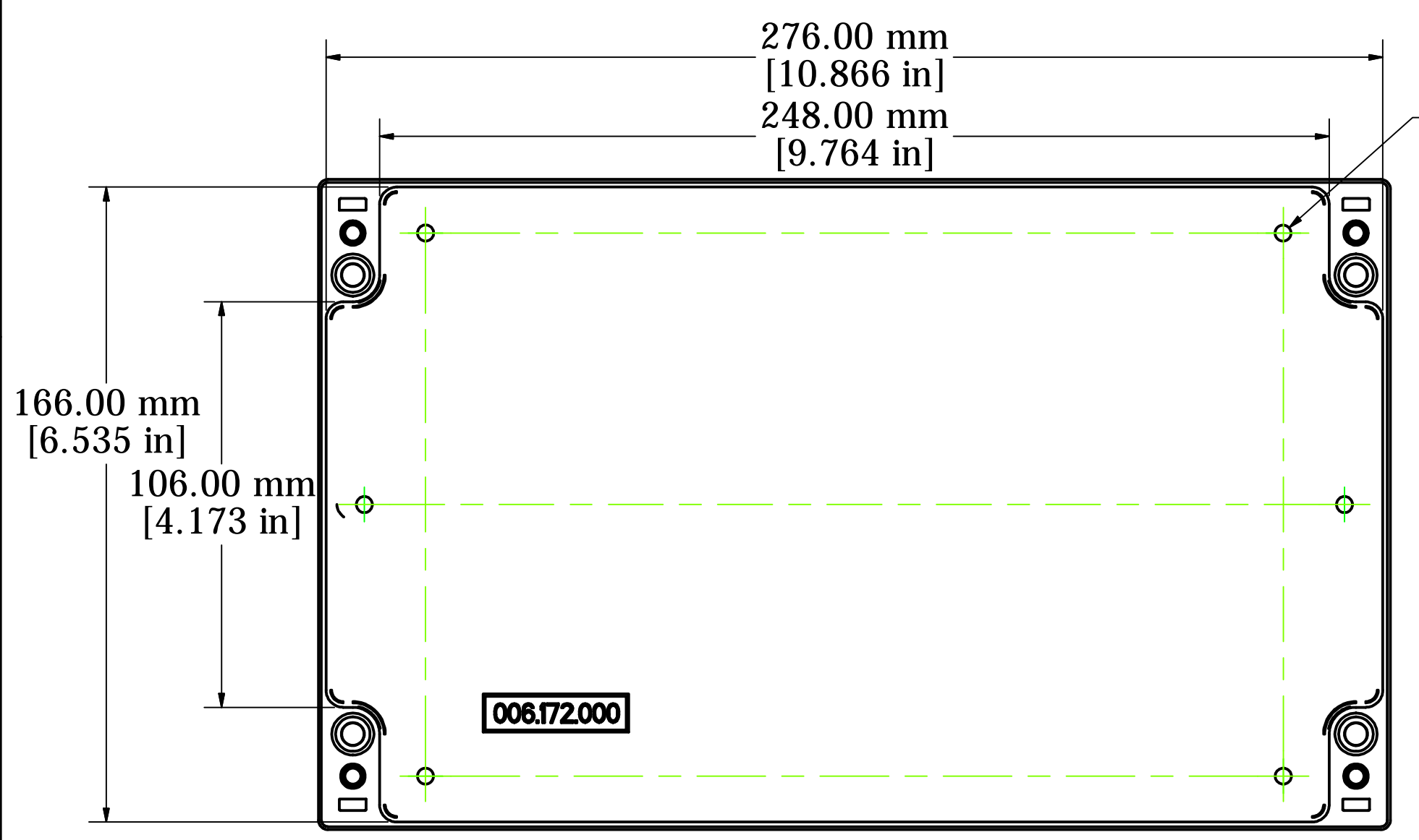
BOX - INSIDE VIEW
