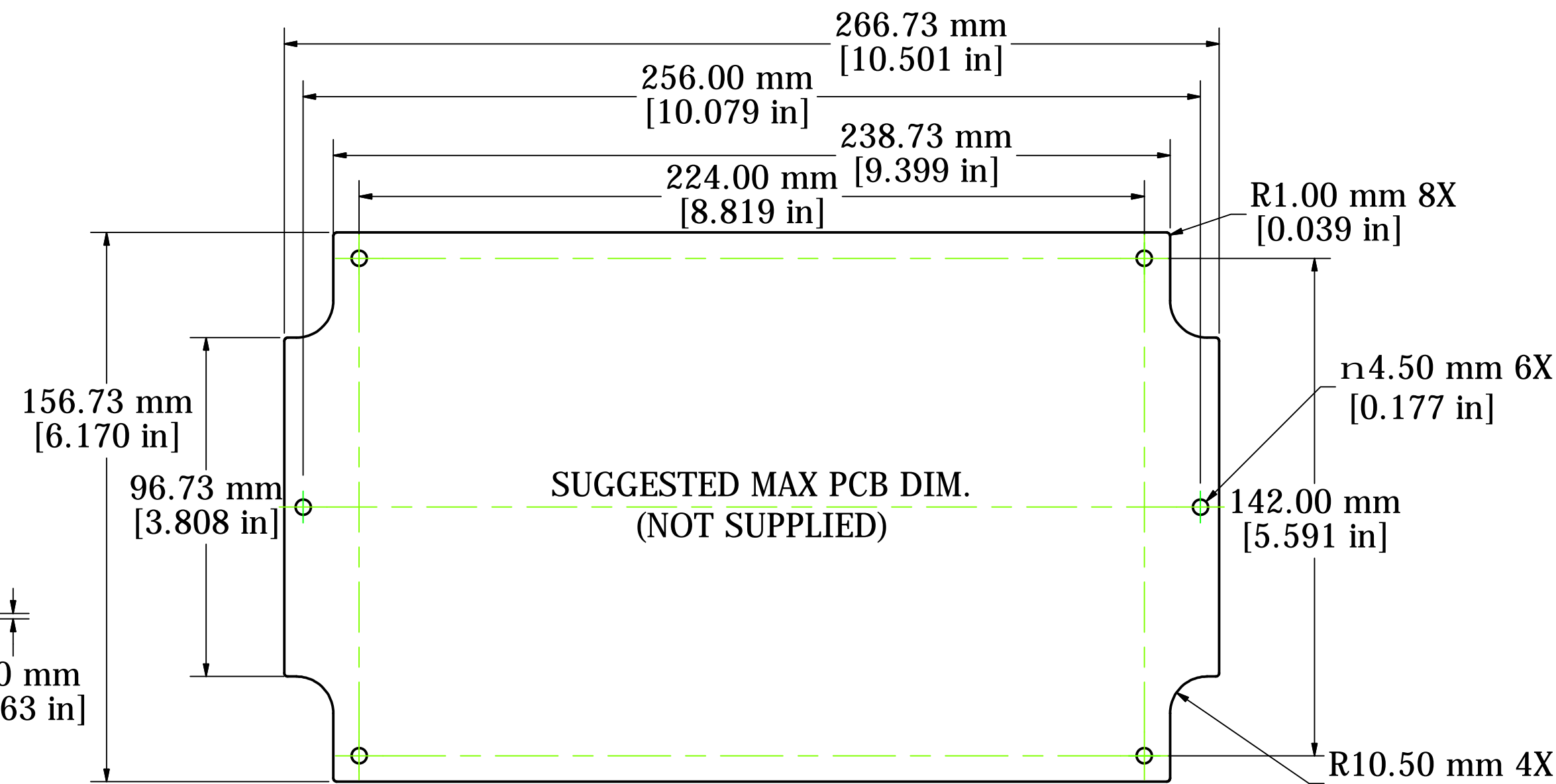
PCB
