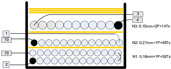
Figure 5—Winding Diagram
