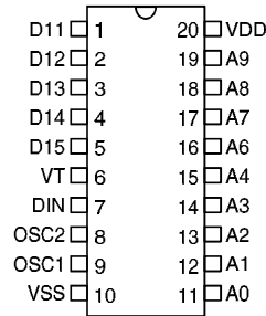
HT605L – 20 DIP/SOP
