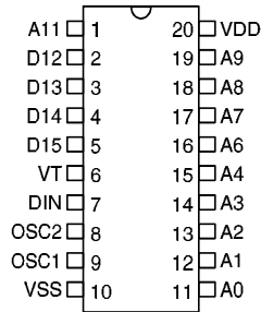
HT604L – 20 DIP/SOP
