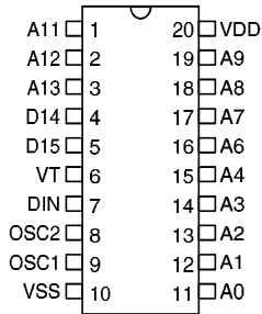
HT602L – 20 DIP/SOP
