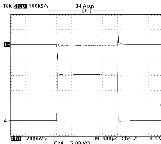
Figure 6 - Transient load response at I_{OUT}=0A - 15A . Ch1: V_{OUT} Ch4: I_{OUT} (5A/div)
