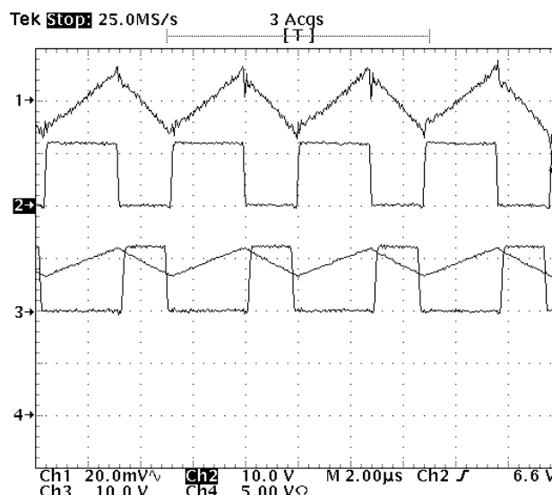
Figure 7 - Normal condition at 15A. Ch1: Output Voltage Ripple (20mV/div) Ch2: HDrv Ch3: LDrv Ch4: Inductor Current (5A/div)
