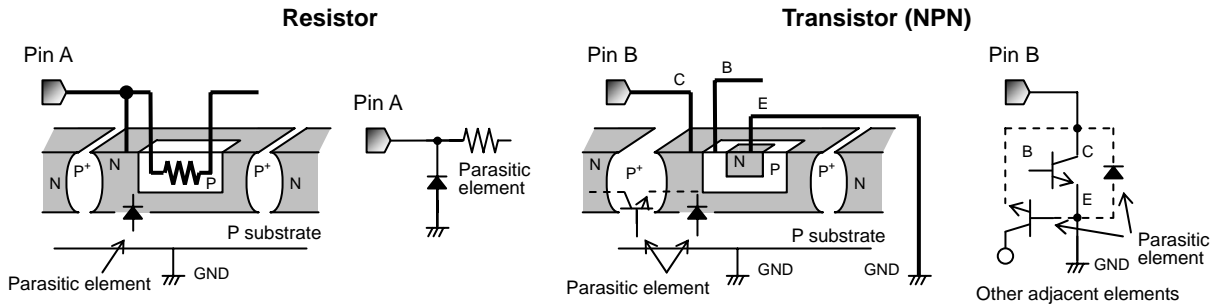
Figure 28. Example of monolithic IC structure
