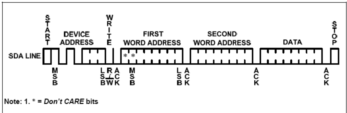
Figure 8 · Byte Write
