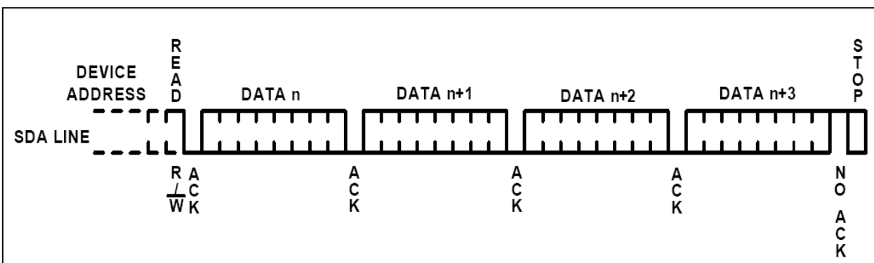
Figure 12 · Sequential Read
