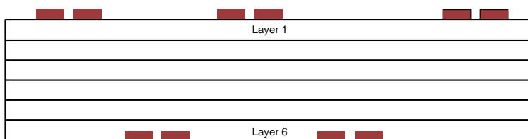
Figure 16. Staggered Trace Layout
