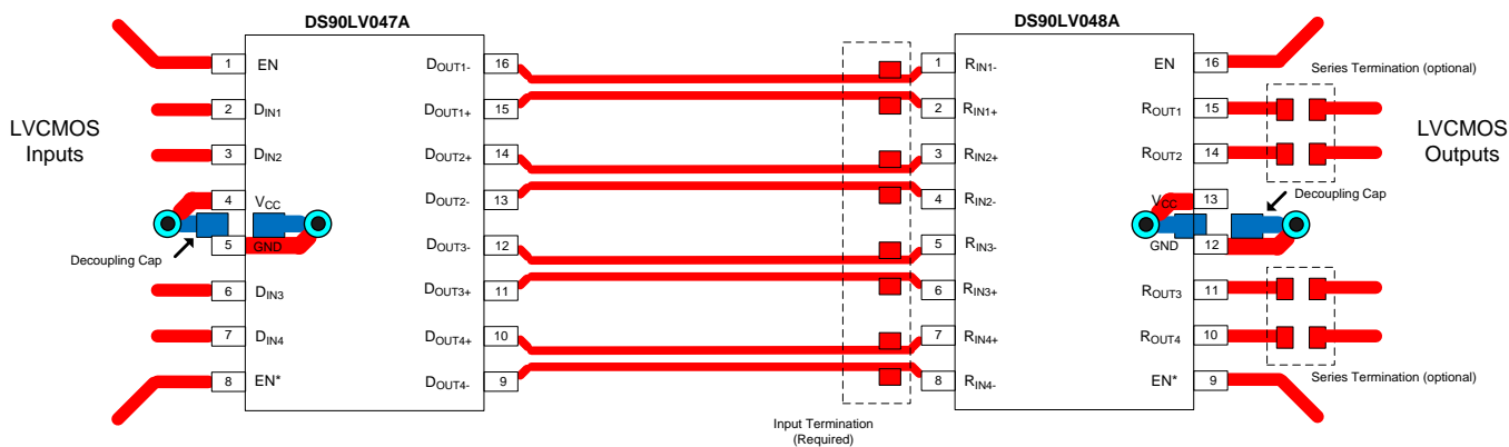
Figure 23. Layout Recommendation
