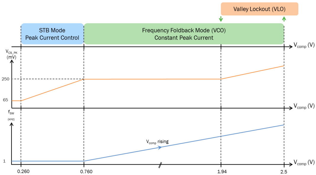
Figure 39. Frequency Foldback and Standby Mode Behavior with 1-kHz Minimum Frequency Clamp, V_{CS(VCO)} = 250\text{ mV} and V_{CS(STB)} = 65\text{ mV}
