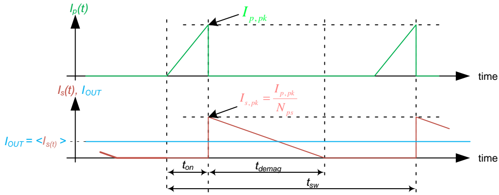
Figure 32. Primary and Secondary Transformer Current Waveforms
