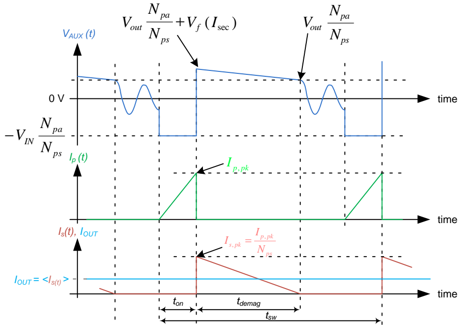
Figure 33. Typical Idealized Waveforms of a Flyback Transformer in DCM
