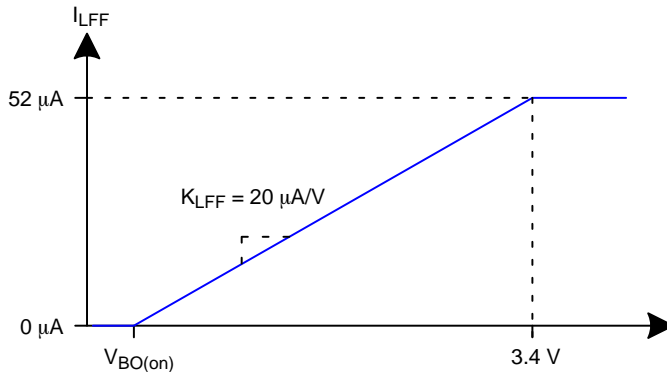
Figure 46. Transfer Function of the Line Feed Forward
