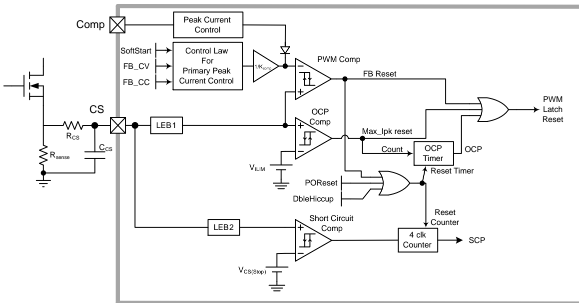
Figure 40. Current Setpoint
