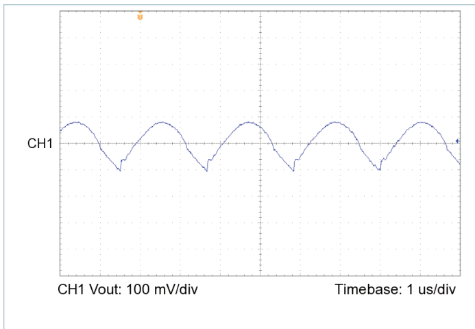
Figure 17 — Output voltage ripple, V_{IN} = 28\text{ V} , V_{OUT} = 5.0\text{ V} , C_{OUT\_EXT} = 1000\ \mu\text{F} , R_{LOAD} = 0.139
