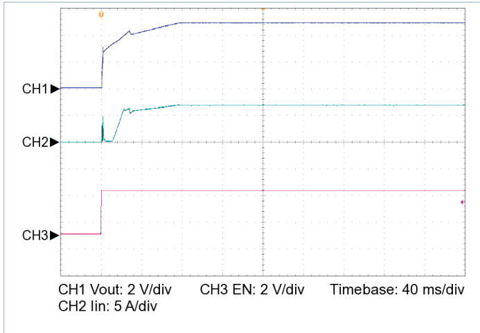
Figure 15 — Startup from EN, V_{IN} = 28\text{ V} , C_{OUT\_EXT} = 20000\ \mu\text{F} , R_{LOAD} = 0.139
