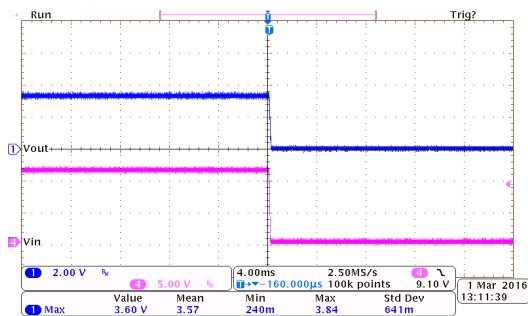
Power Off Response: HT7333-7 ( I_{OUT}=250mA , T_{FALL}=0.1ms )
