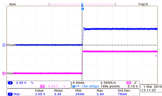
Power On Response: HT7333-7 ( I_{OUT}=250mA , T_{RISE}=0.1ms )
