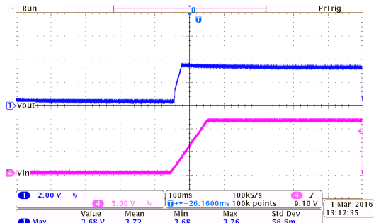
Power On Response: HT7333-7 ( I_{OUT}=0mA , T_{RISE}=100ms )
