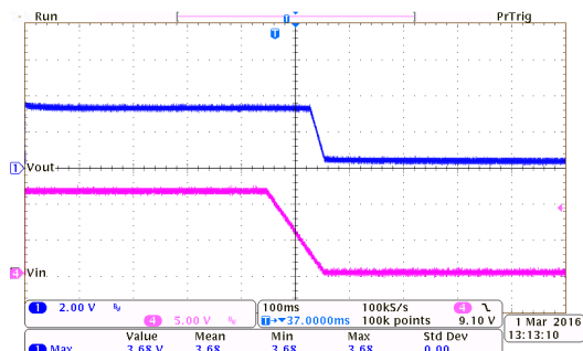
Power Off Response: HT7333-7 ( I_{OUT}=0mA , T_{FALL}=100ms )
