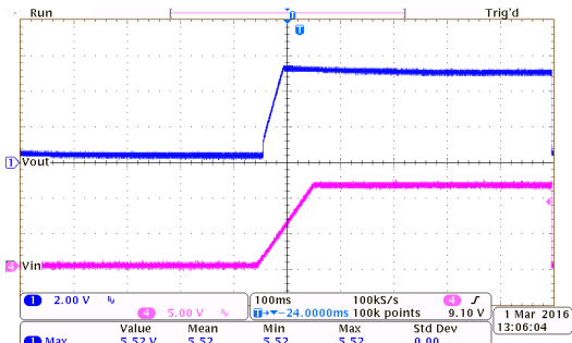
Power On Response: HT7350-7 ( I_{OUT}=0mA , T_{RISE}=100ms )
