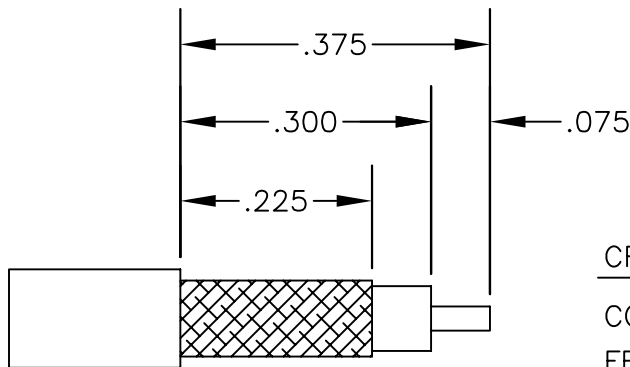
STRIPPING DIMENSIONS
