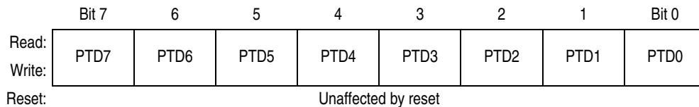
Figure 11-13. Port D Data Register (PTD)
