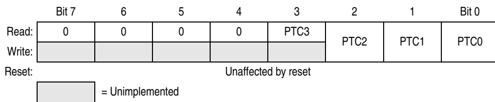
Figure 11-9. Port C Data Register (PTC)
