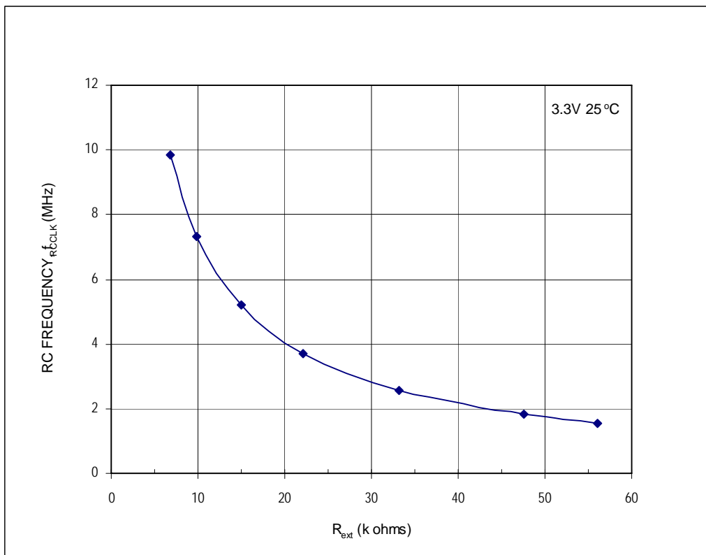
Figure 19-8. RC versus Frequency (3.3 Volts @ 25°C)
