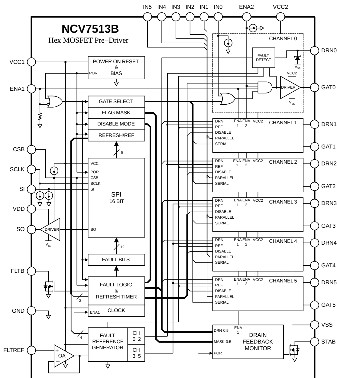
Figure 1. Block Diagram
