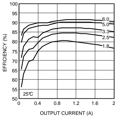
Figure 11. Efficiency 20-V Input at 25°C
