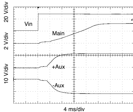
4 ms/div Full resistive load, 28 V_{IN} SMRT283R312T Representative of Triple Output Turn On Delay FIGURE 51
