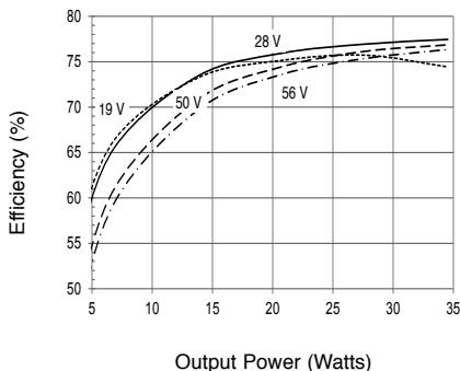
SMRT2805S Efficiency FIGURE 19
