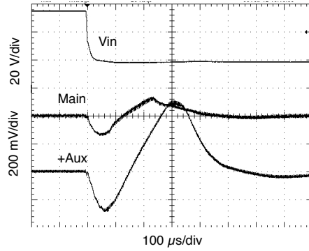
100 \mu s/div Vin 56 to 19 V, full resistive load SMRT283R312T Representative of Triple Output Line Transient FIGURE 48
