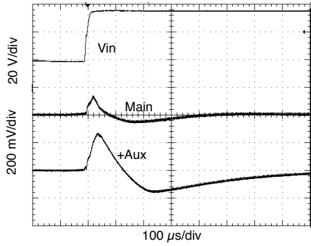
100 \mu s/div Vin 19 to 56 V, full resistive load SMRT283R312T Representative of Triple Output Line Transient FIGURE 47
