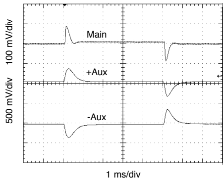
1 ms/div Load 50 - 100 - 50%, 50 V_{IN} SMRT283R312T Representative of Triple Output Load Transient FIGURE 50
