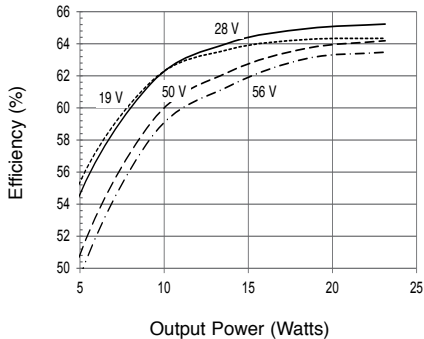
SMRT283R3S Efficiency FIGURE 17
