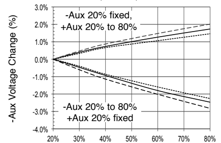
+Aux Load (%), 28 V_{IN} ..... -55°C — 25°C - - 125°C SMRT28515T Cross Regulation FIGURE 55
