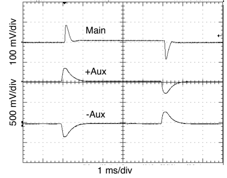
1 ms/div Load 50 - 100 - 50%, 28 V_{IN} SMRT283R312T Representative of Triple Output Load Transient FIGURE 49
