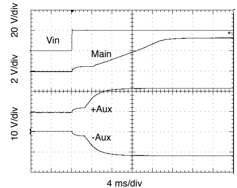
4 ms/div Full resistive load, 50 V_{IN} SMRT283R312T Representative of Triple Output Turn On Delay FIGURE 52
