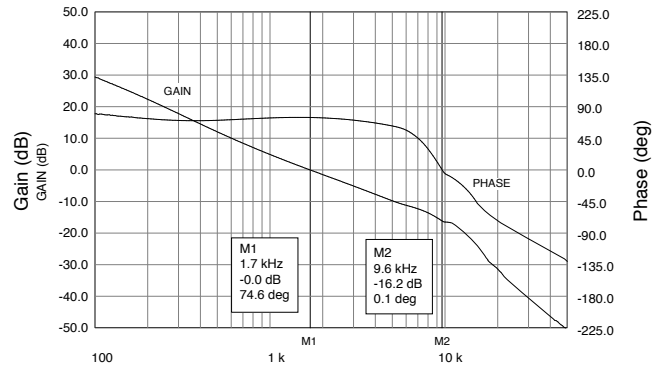
SMRT2812S Gain Phase FIGURE 24
