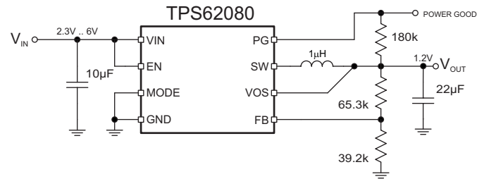
Figure 34. 1.2V Output Voltage Application (TPS62080)
