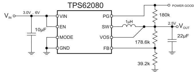
Figure 35. 2.5V Output Voltage Application (TPS62080)
