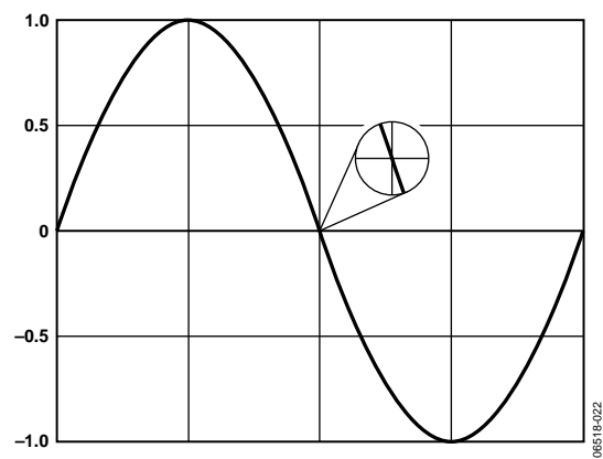
Figure 49. Maximum Slew Rate of a Sine Wave with an Amplitude of 2 V p-p
