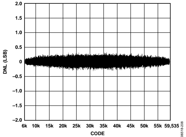
Figure 24. DNL Plot
