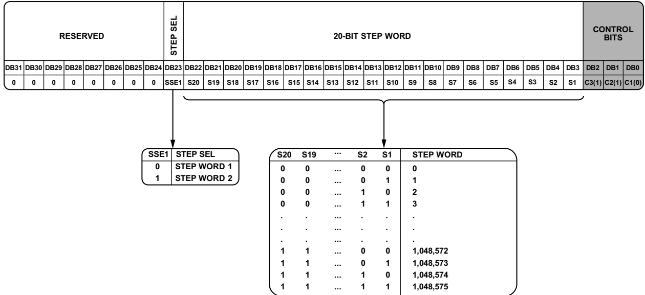
Figure 31. Step Register (R6) Map
