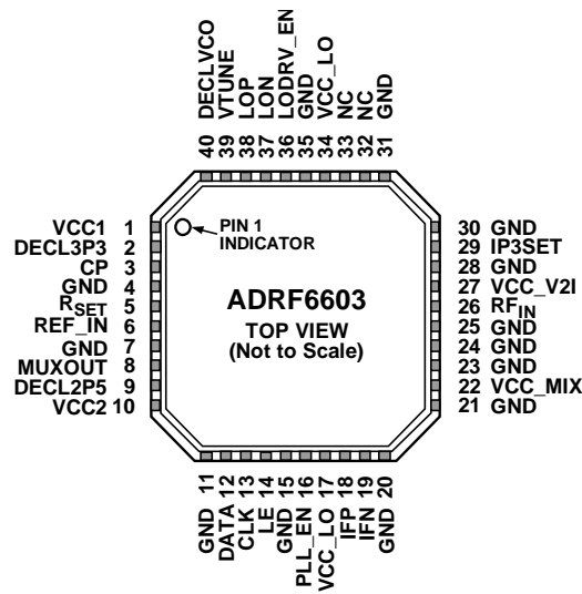
Figure 3. Pin Configuration
