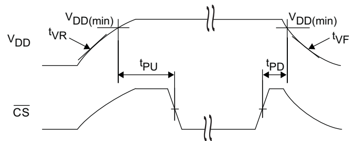
Figure 18. Power Cycle Timing
