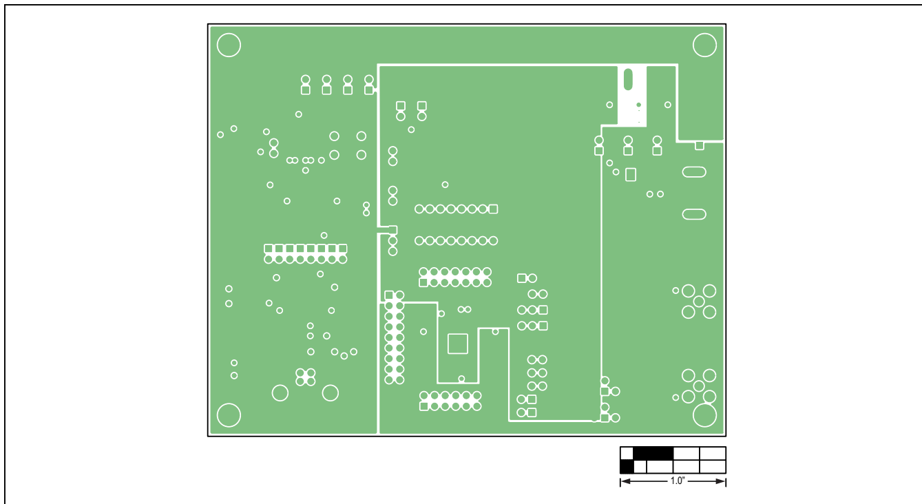
Figure 14. MAX9273 Coax EV Kit PCB Layout—Power Layer 3
