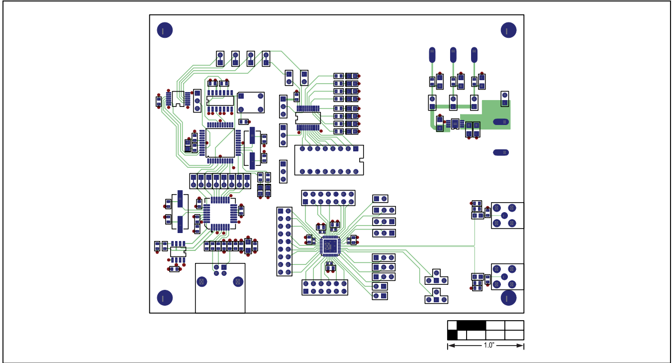
Figure 12. MAX9273 Coax EV Kit PCB Layout—Component Side
