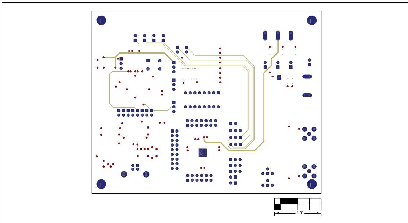
Figure 15. MAX9273 Coax EV Kit PCB Layout—Solder Side
