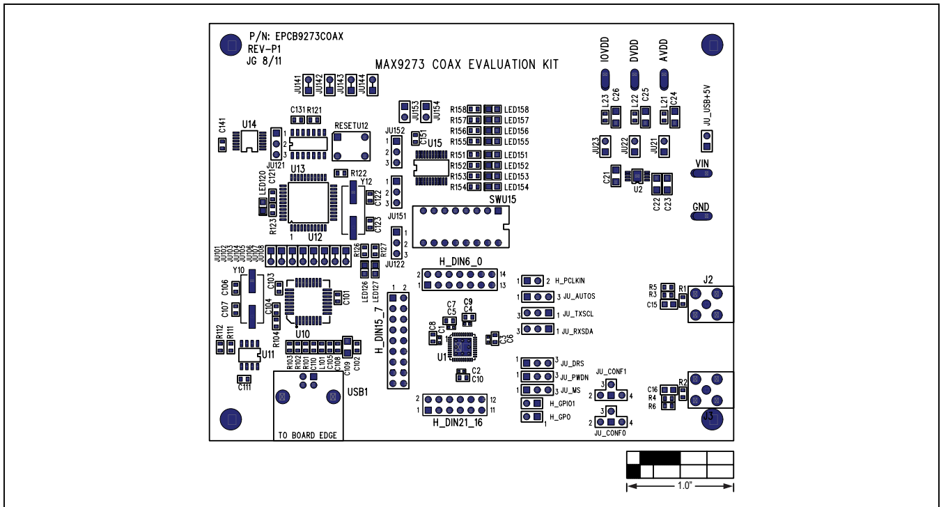
Figure 11. MAX9273 Coax EV Kit Component Placement Guide—Component Side
