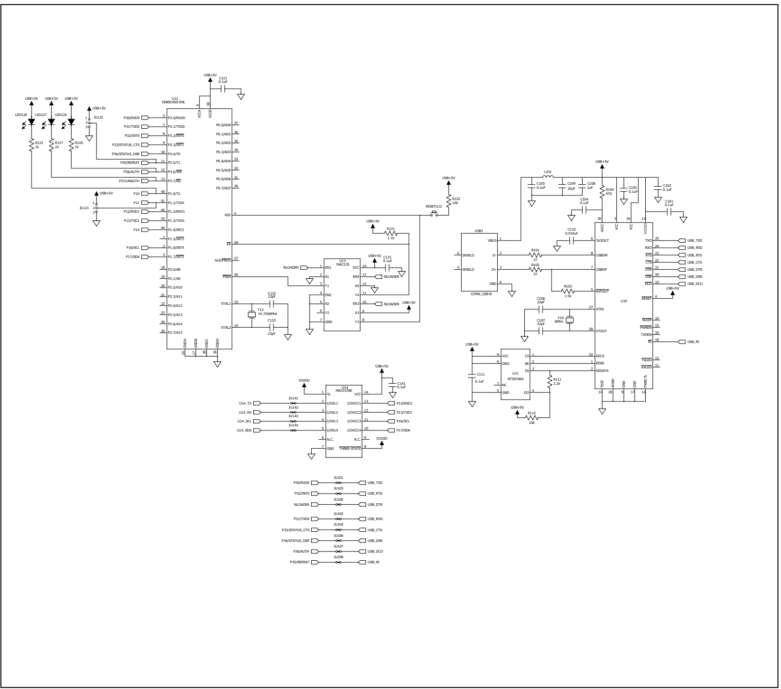
Figure 10b. MAX9273 Coax EV Kit Schematic (Sheet 2 of 3)
