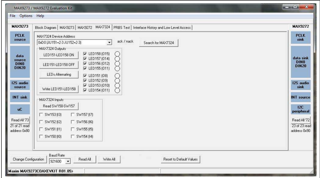
Figure 4. MAX9273/MAX9272 EV Kit Software Main Window (MAX7324 Tab)
