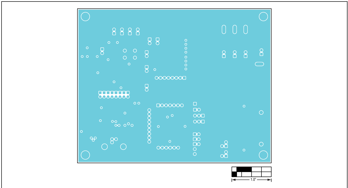
Figure 13. MAX9273 Coax EV Kit PCB Layout—Ground Layer 2
