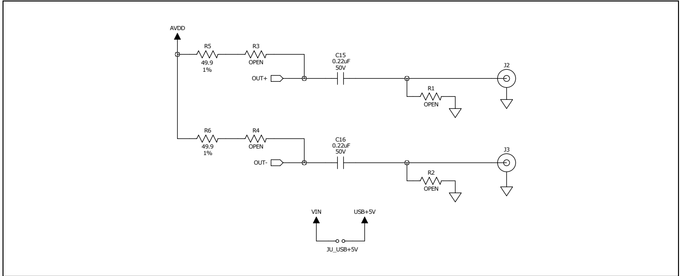
Figure 10c. MAX9273 Coax EV Kit Schematic (Sheet 3 of 3)
