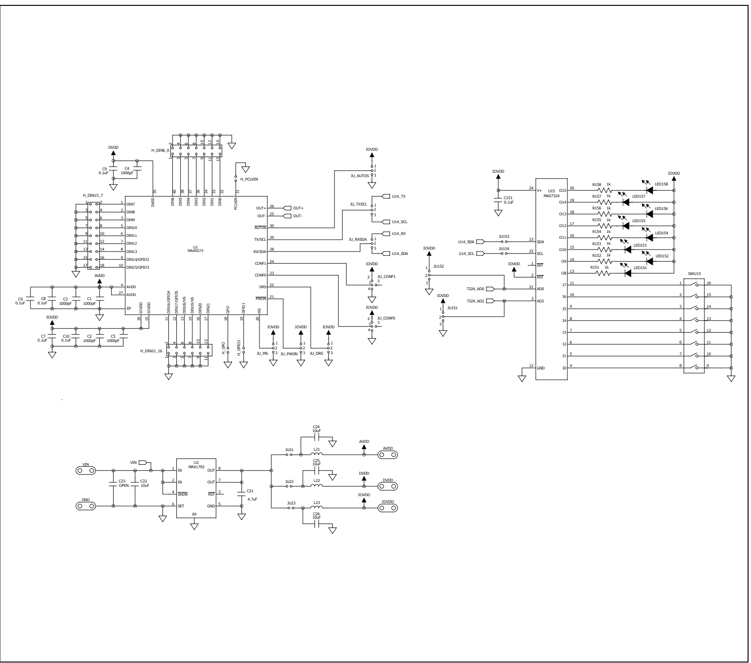
Figure 10a. MAX9273 Coax EV Kit Schematic (Sheet 1 of 3)
