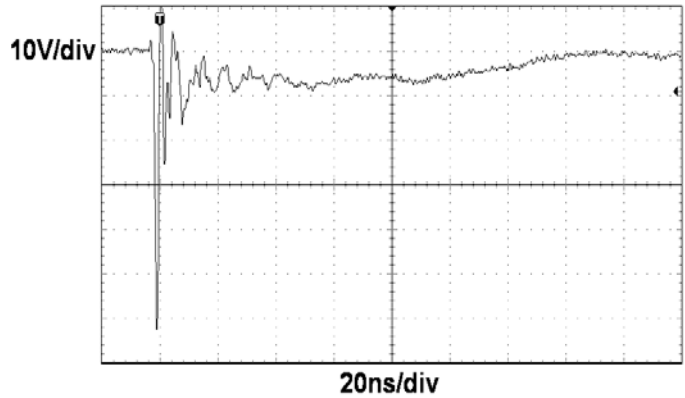
ESD clamping (-8kV contact discharge per IEC61000-4-2)
