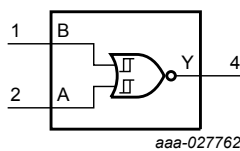
Figure 1. Logic symbol
