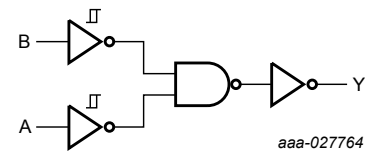
Figure 3. Logic diagram
